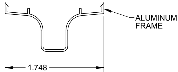
CROSS-SECTION VIEW
